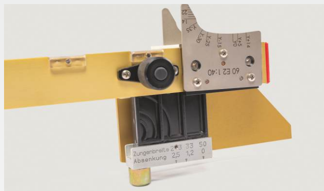
Rail head profile template, rail head width scale and frog inclination measuring unit (option)
